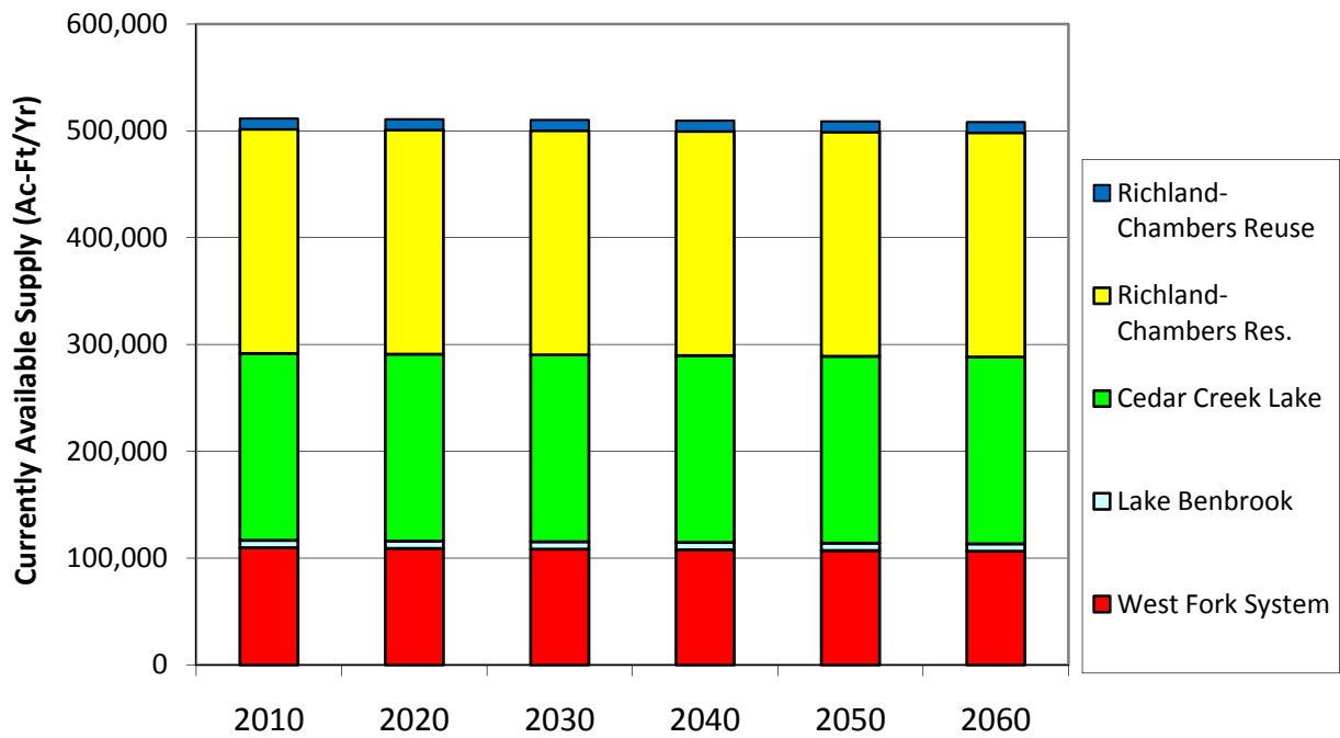
Figure 3.4 Currently Available Water Supplies for the Tarrant Regional Water District
